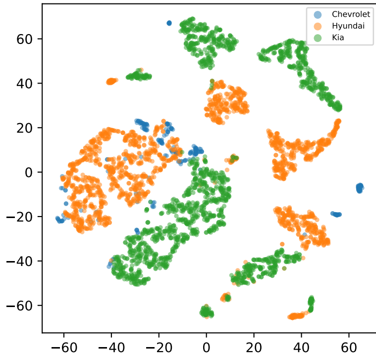
t-SNE — Vehicle model
