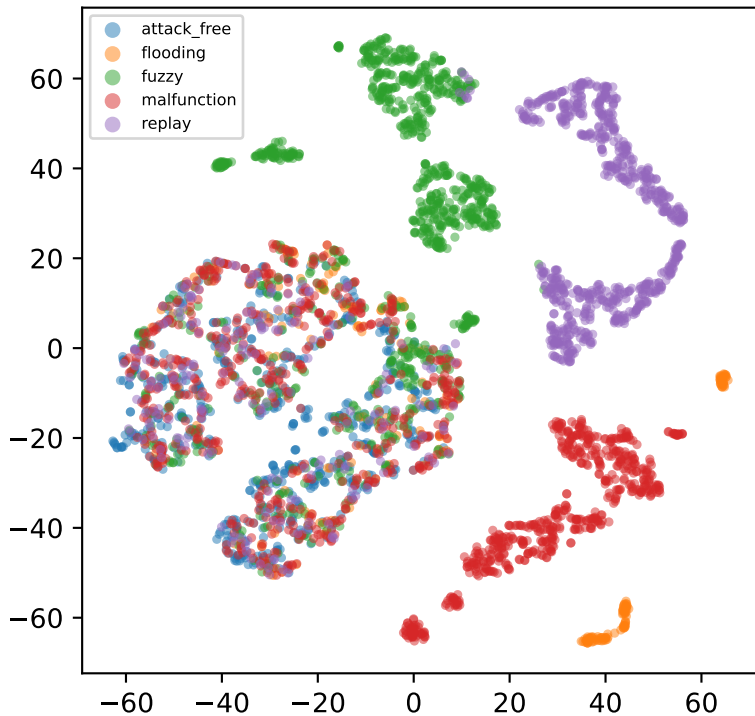
t-SNE — Attack type
