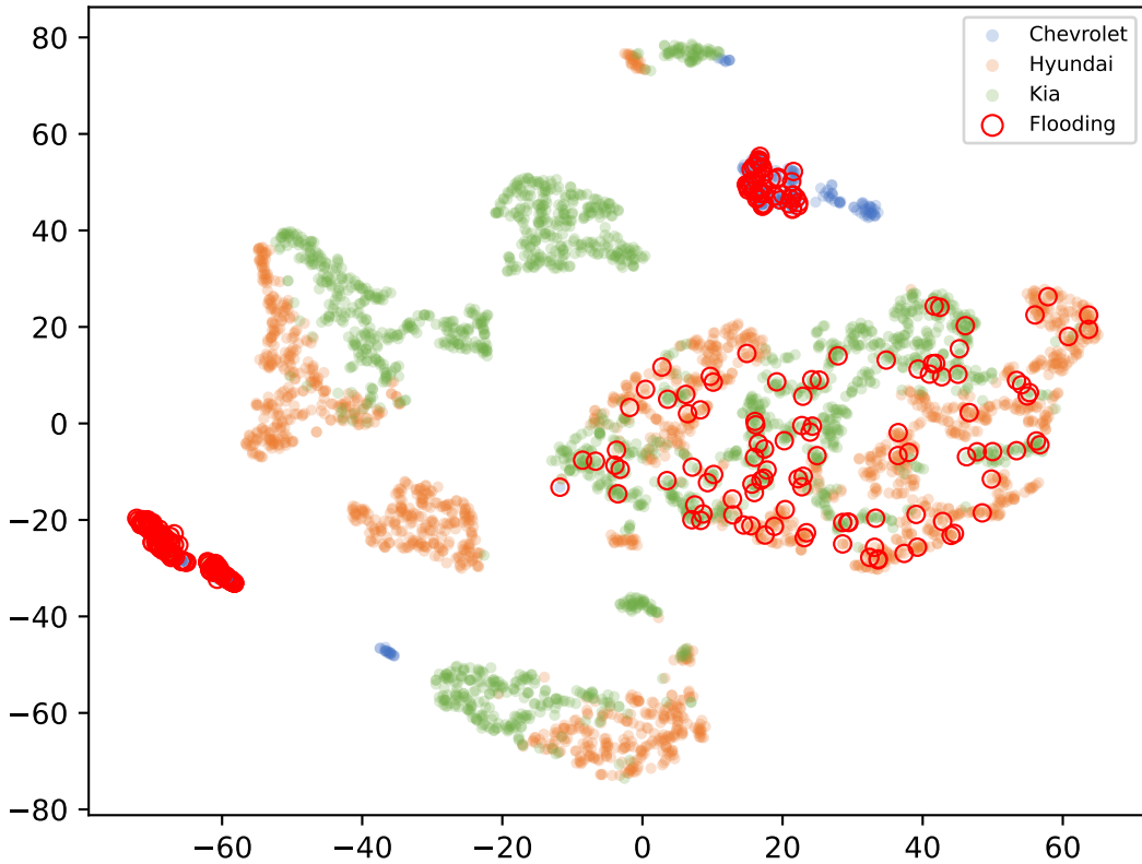
Behaviour-Only Descriptor Embedding (t-SNE)
