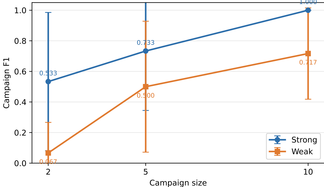
Strong vs weak coordinated-campaign F1 (balanced OCSLab)
