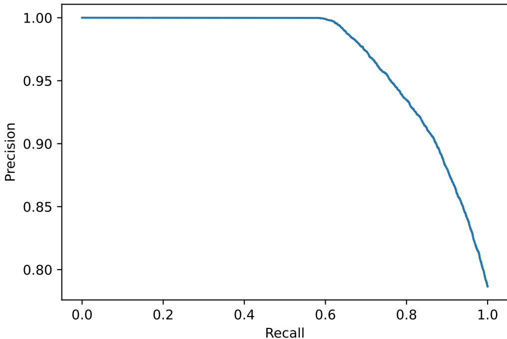
Vehicle-level precision-recall
