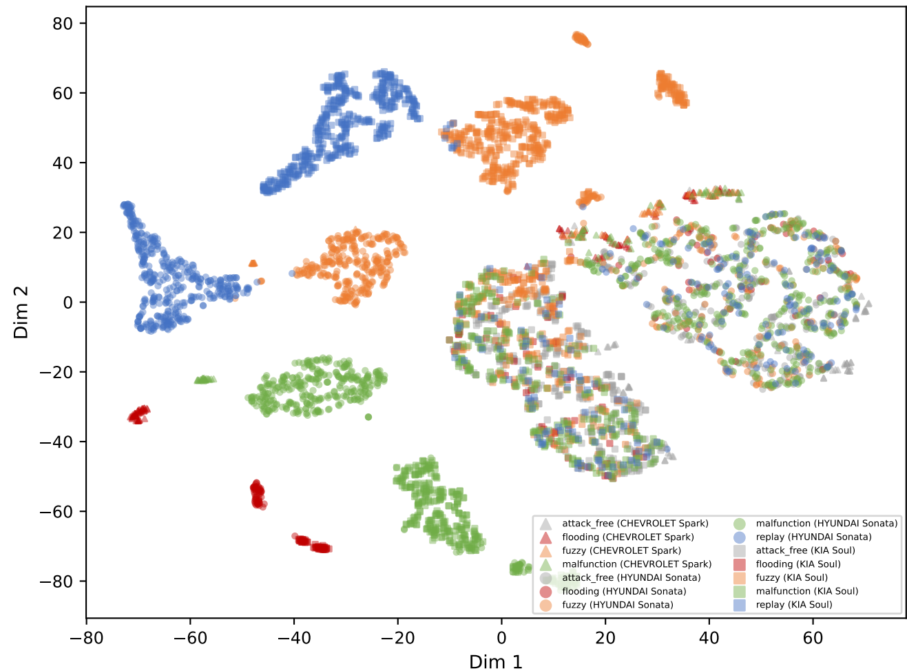
Descriptor embedding — colour: attack type, marker: vehicle
