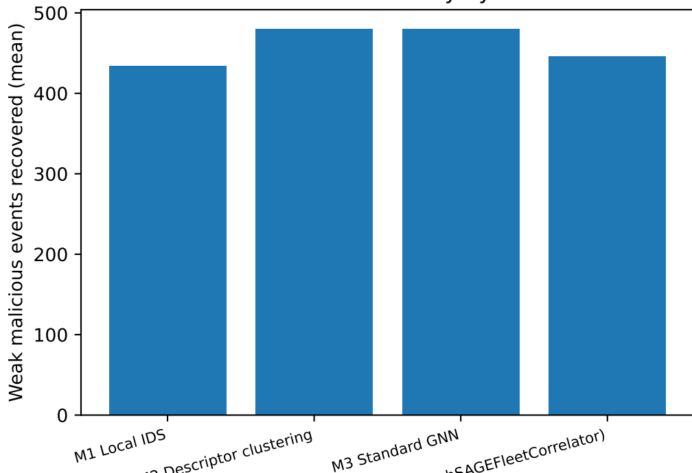
S4 weak-event recovery by method
