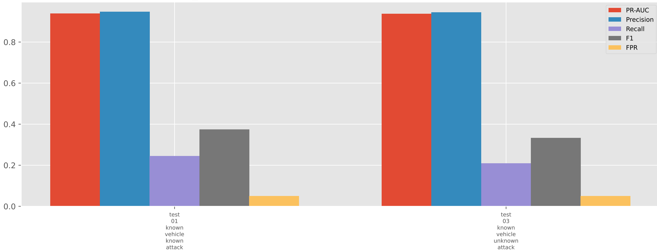
LOCAL_COMP5 — CTT local IDS by subset (available subsets only)
