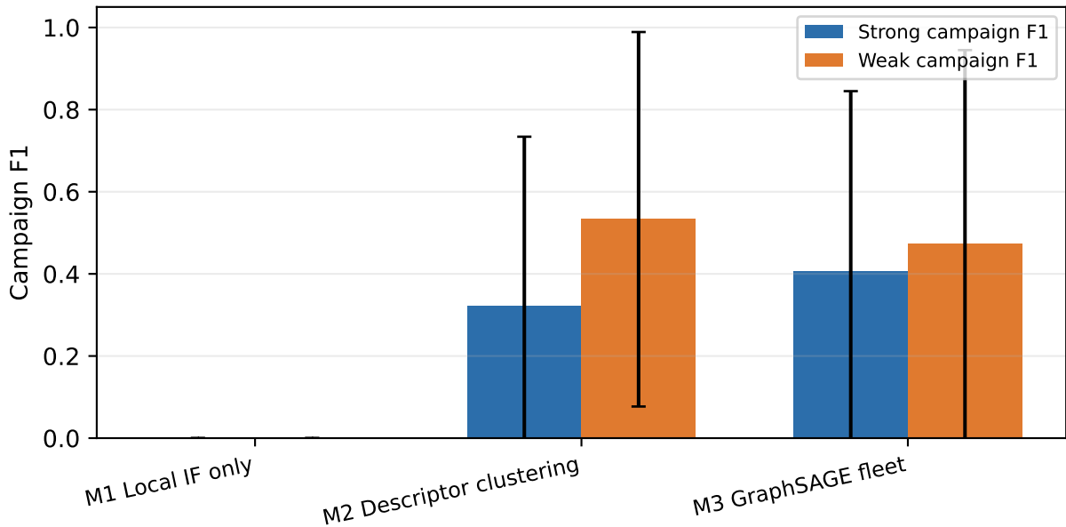
Baseline / ablation: coordinated campaign F1
