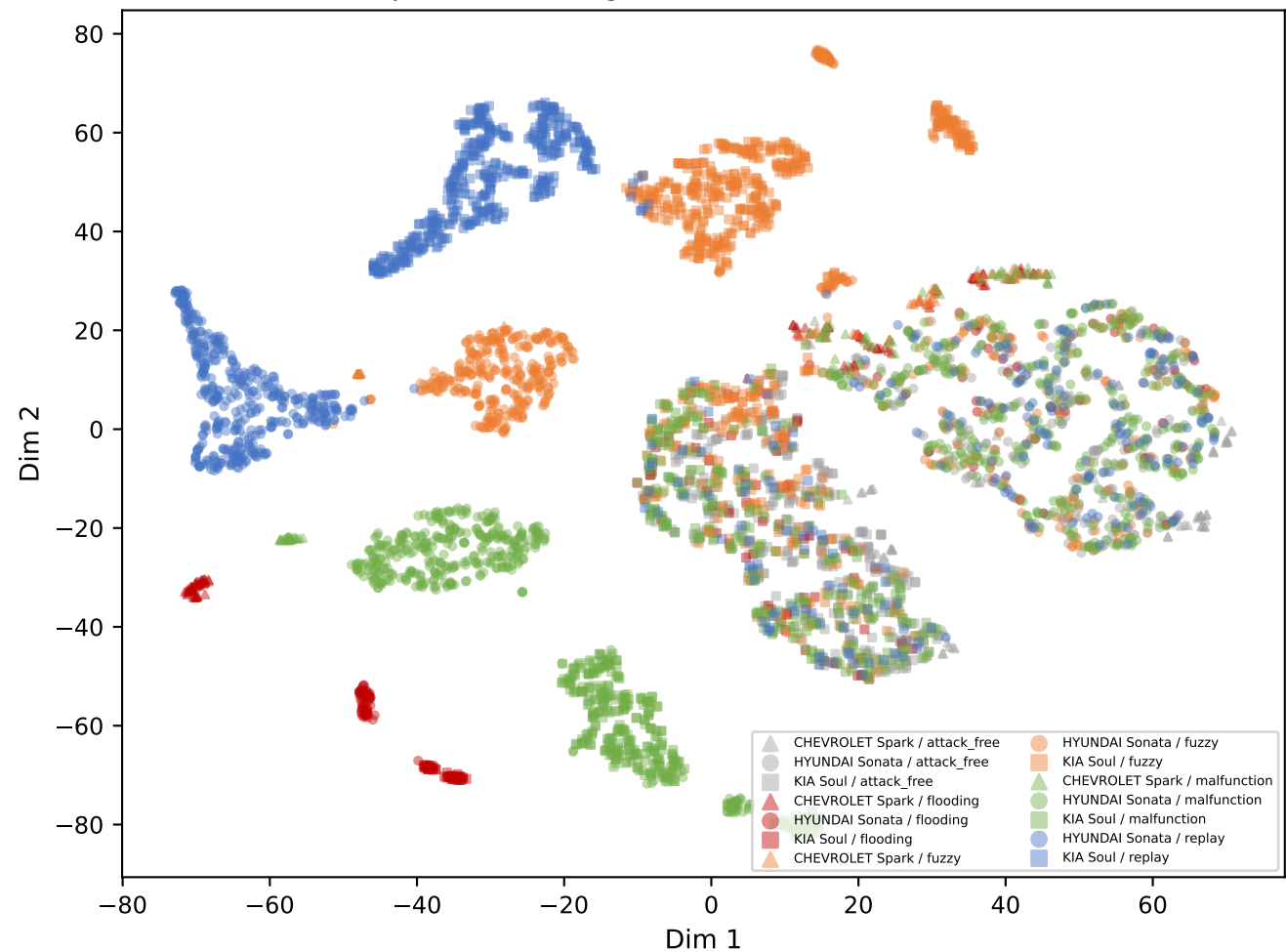
Descriptor embedding — colour: attack, marker: vehicle
