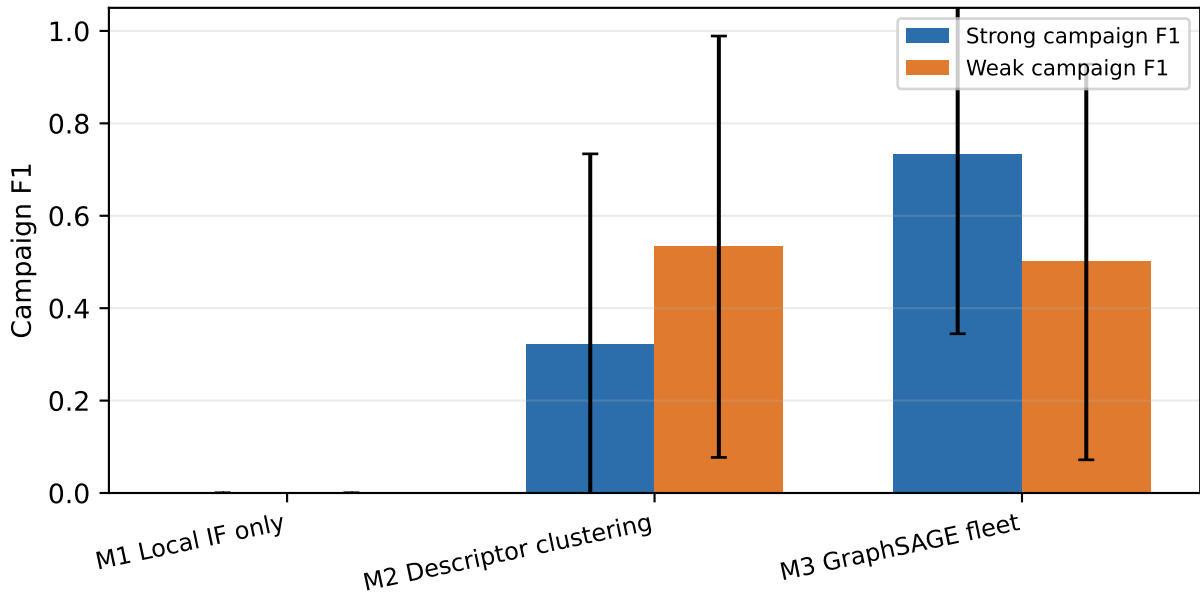
Baseline / ablation: coordinated campaign F1
