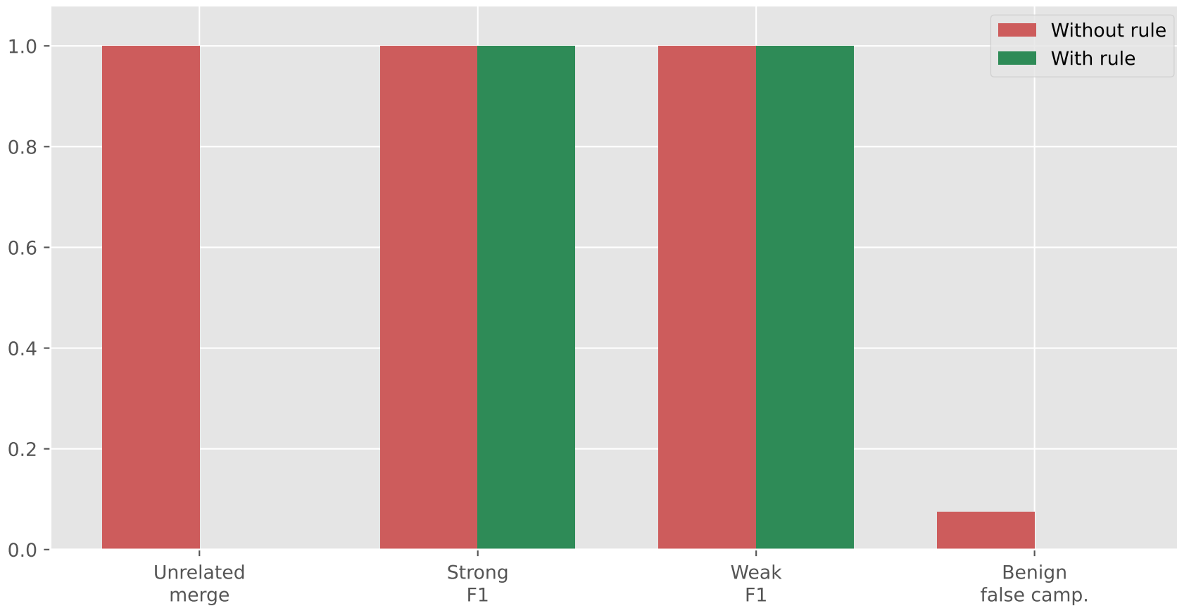
Campaign consistency rule ablation (CTT)
