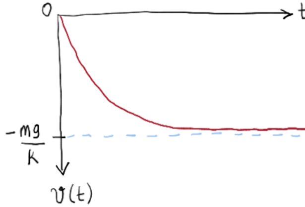
Figure 4: Velocity of a particle falling under gravity with air resistance proportional to its velocity. The velocity approaches the terminal speed v_{\text{terminal}} = \frac{mg}{k} as t \rightarrow \infty .
