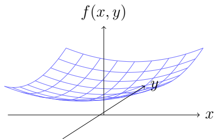
Figure 2: The surface f(x, y) = x^2 + y^2 .
