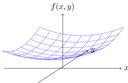
Figure 2: The surface f(x, y) = x^2 + y^2 .
