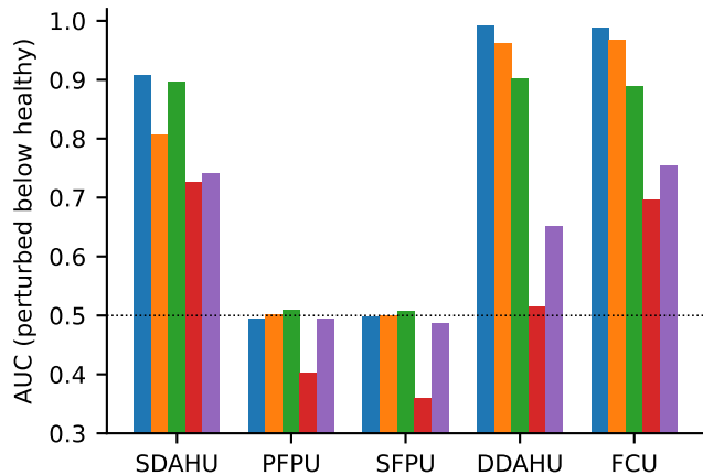
Threshold-free separability
