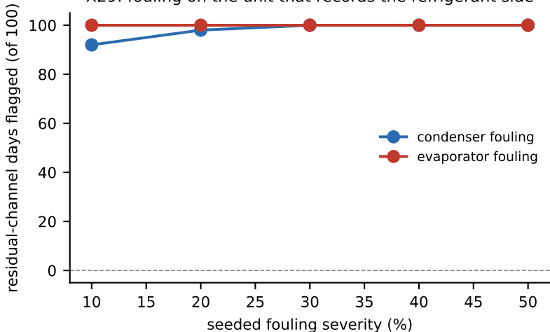
X29: fouling on the unit that records the refrigerant side
