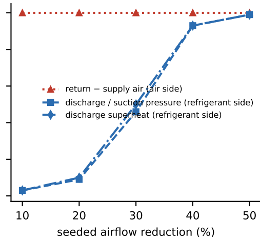
Evaporator fouling
