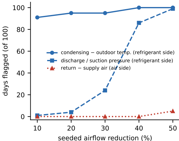
Condenser fouling
