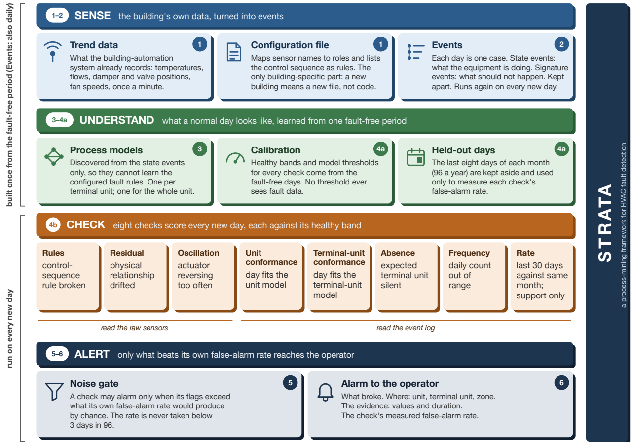
Fig. 1. The STRATA framework as four tiers. The top two tiers are built once per building from one fault-free period: the trend data is turned into events, process models of a normal day are discovered from the state events, and the eight checks are calibrated, with their false-alarm rates measured on held-out days. The bottom two tiers run on every new day, after the day has been turned into events by the same Stage 2 rules: the eight checks score it, the noise gate passes only alarms that beat the check's own false-alarm rate, and what passes reaches the operator stating what broke, where, the evidence and that rate. The numbered badges are the stages of Section II; 4a (calibration) and 4b (the checks) are the two halves of Stage 4.
