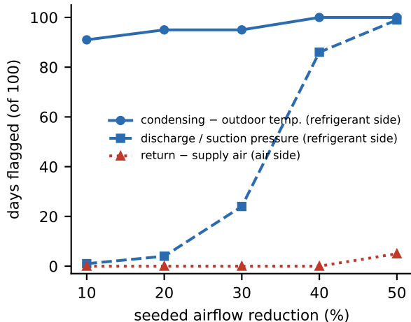
Condenser fouling
