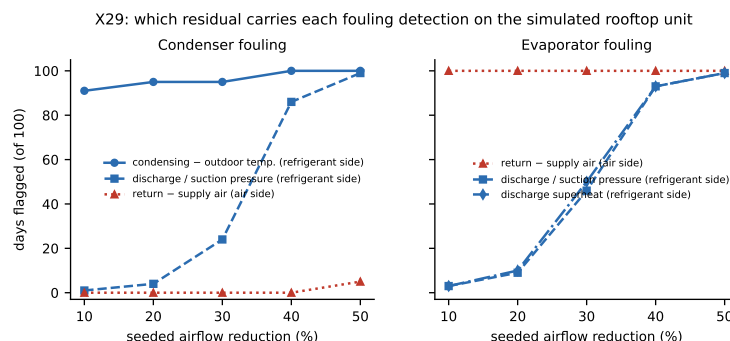
Figure 6. Which residual carries each fouling detection on the simulated rooftop unit, by seeded airflow reduction (days flagged of 100, from the per-residual credit artefact). Condenser fouling is carried by the refrigerant-side condensing-temperature approach at every severity; evaporator fouling is carried by the air-side return-minus-supply residual at every severity, with the refrigerant-side residuals joining from 30%.
