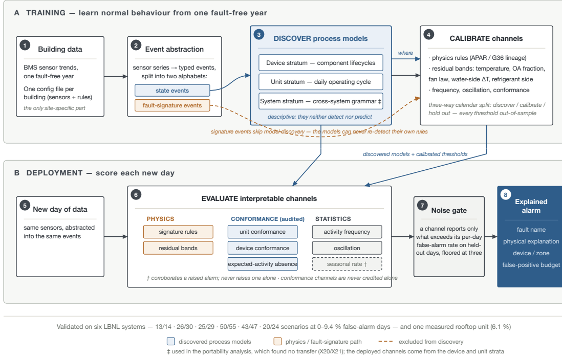
Figure 1: The framework as evaluated. Training (top): one fault-free year and one configuration file; events split into state and fault-signature alphabets; process models discovered from state events only; every threshold from a three-way calendar split (discover, calibrate, hold out), so every reported false-alarm rate is out-of-sample. Deployment (bottom): each day is scored by physics, statistical and conformance channels, each reporting only what exceeds its own per-day false-alarm rate; what survives reaches the operator with a name, a physical explanation, the device and the stated budget.
