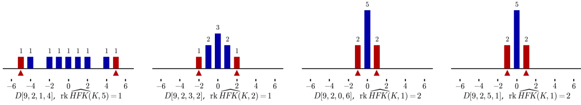
FIGURE 18. The groups \widehat{\text{rkHFK}}(K, s) of the four diagrams of Figure 17 on one pair of axes, the columns and the marks at s = \pm A_{\text{top}} in red, so that the gaps of the \bowtie staircase, the single top of S \neq 0 and the three levels of S = 0 are read side by side.
