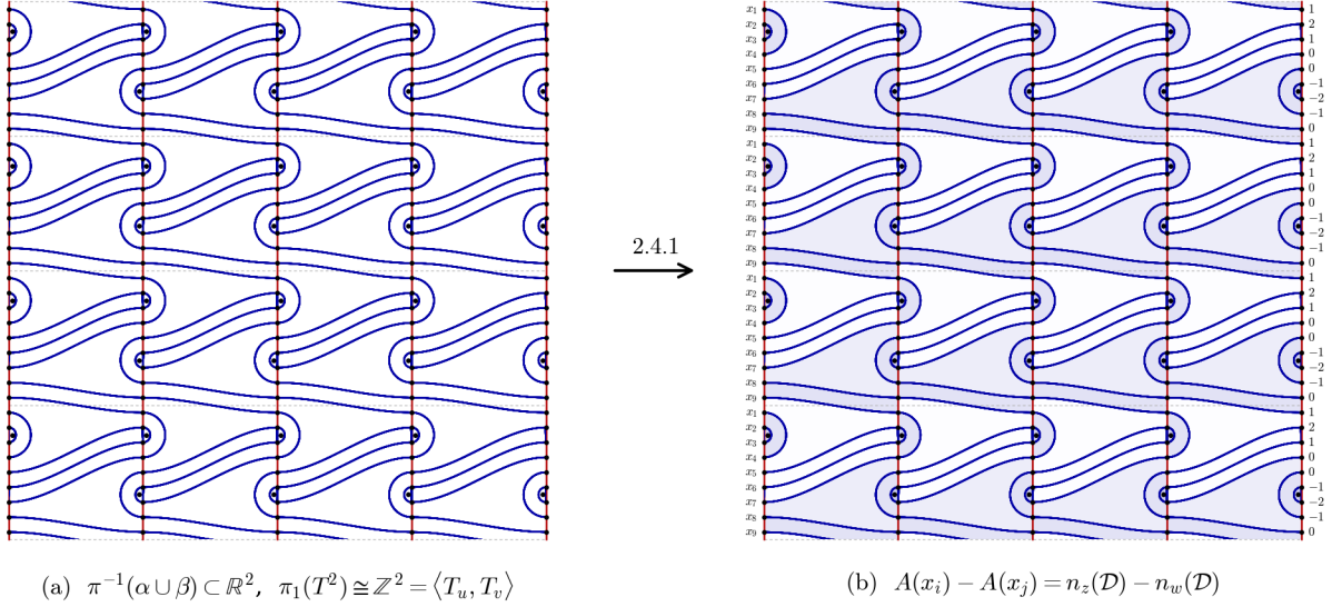
FIGURE 13. The cover of D[9, 2, 3, 2] , type B, read the same way through Definition 2.3.1, giving A = (1, 2, 1, 0, 0, -1, -2, -1, 0) .
