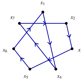
FIGURE 8. The traversal of D[7, 2, 1, 3] as the 7-cycle (1472356) .
