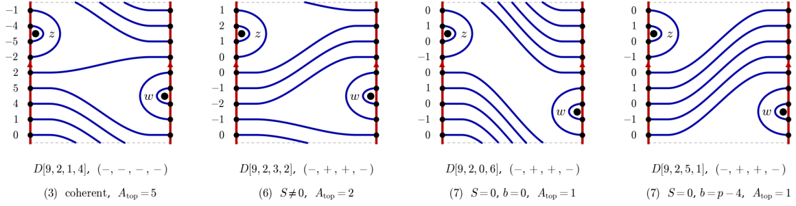
FIGURE 17. The four cases of Theorem 3.0.1 at p = 9 , each drawn on the annulus T^2 \setminus \alpha whose two red edges are glued by \downarrow \downarrow , with the sign word (\eta(O_L), \eta(O_R), \eta(I_L), \eta(I_R)) printed beneath and the number beside a foot equal to A(x_h) .
