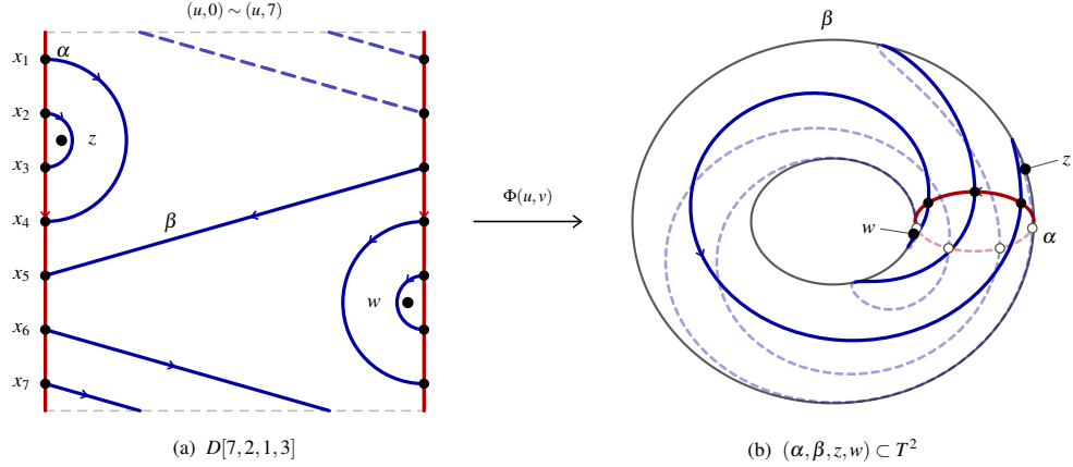
FIGURE 2. [7, 2, 1, 3] as in Figure 1, with two returns round the meridian. Coherent, e = +1 .
