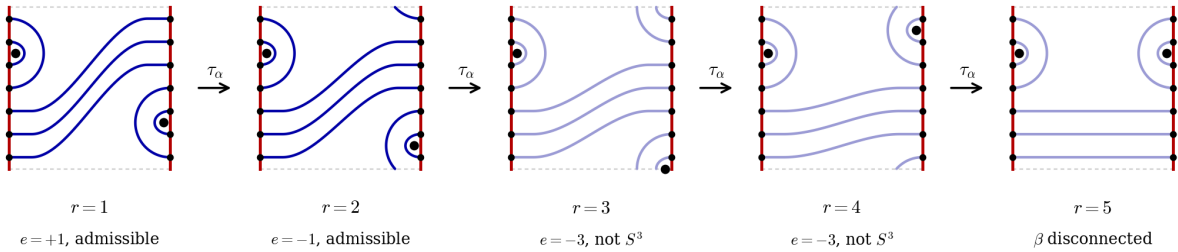
FIGURE 16. The \langle \tau_\alpha \rangle -orbit of D[7, 2, 3, 1] : the sign of e flips, then |e| \neq 1 , then \beta disconnects.
