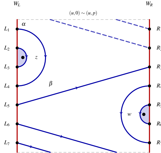
FIGURE 5. \mathcal{D}[7, 2, 1, 3] with v = 4 , the nests O_L = L_1L_4 \supset I_L = L_2L_3 and O_R = R_4R_7 \supset I_R = R_5R_6 cutting off \mathcal{D}_z, \mathcal{D}_w , the band \mathcal{B} = \{L_5R_3\} , and the returns L_6R_1, L_7R_2 crossing (u, 0) \sim (u, p) with their second pieces dashed. Under \downarrow \uparrow the slots L_h, R_h have common image x_h .
