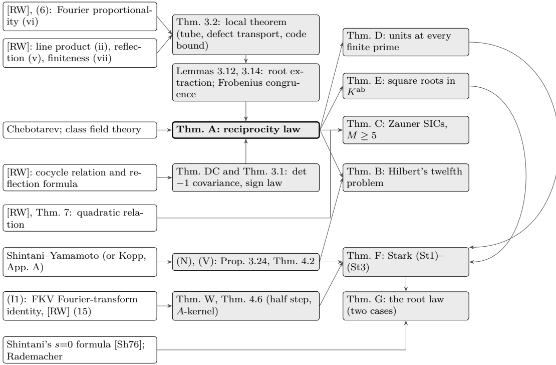
FIGURE 1. Dependencies among the main results. Boxes on the left are imported results, boxes in the middle are the new arguments, and boxes on the right are the main theorems. Theorem G also uses further identities of [RW] (Section 4.5).
