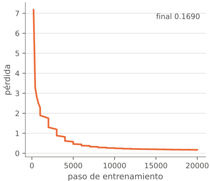
ACT
