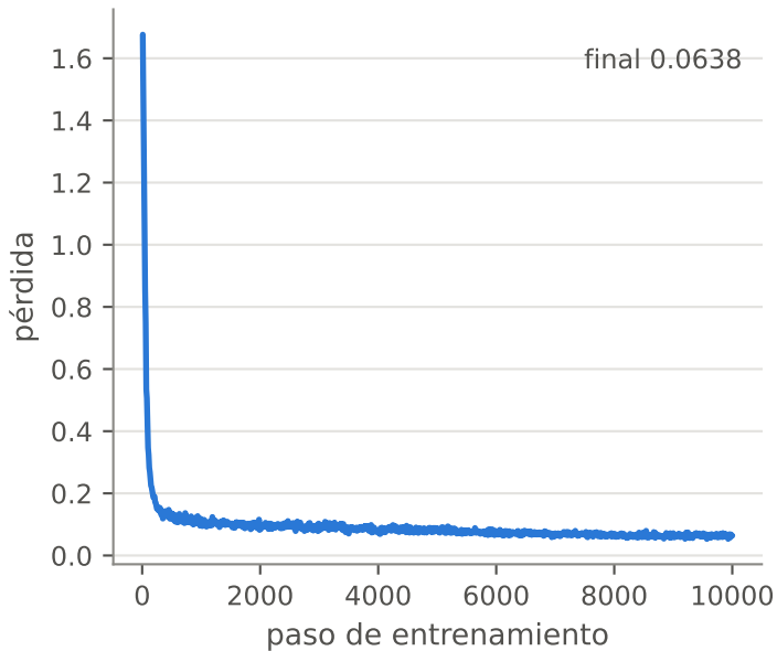
GR00T
