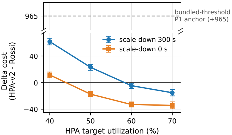
Rossi P1 under HPA-v2 configuration sensitivity
