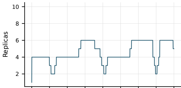
HPA-v2 clean
