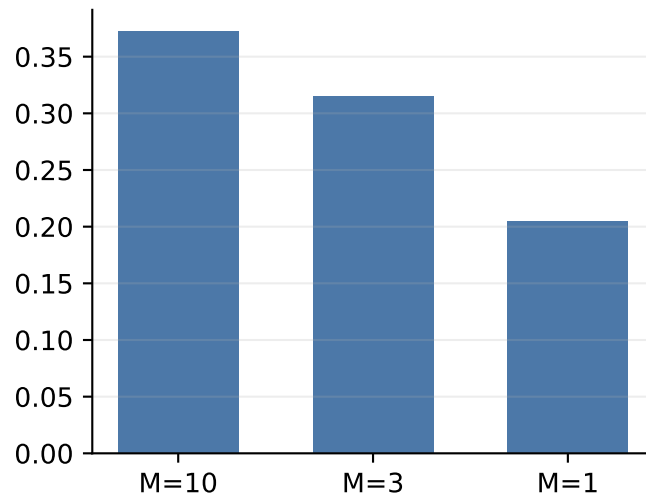
Total variation
