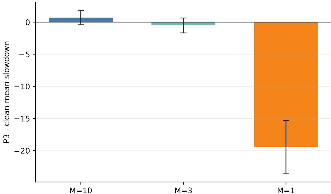
DeepRM FGSM degradation by visible action set
