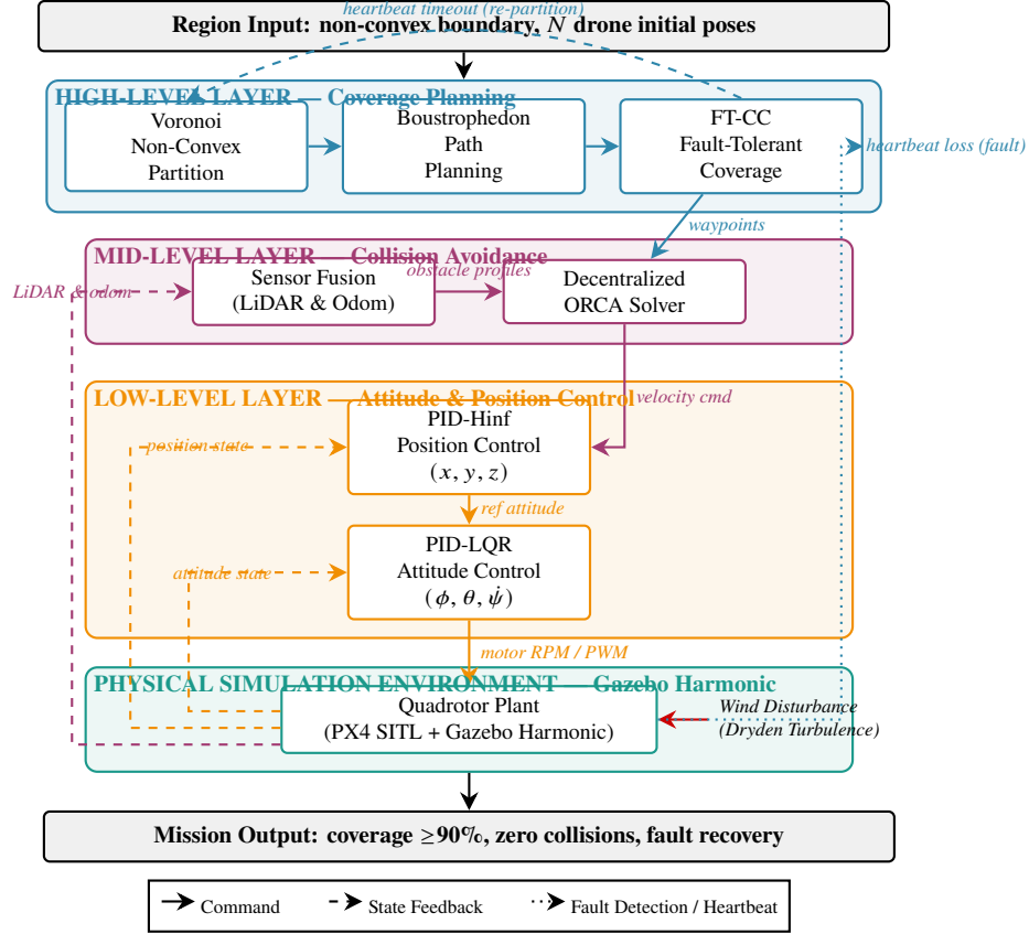
Figure 1 Proposed three-layer control architecture for resilient autonomous swarm quadrotor geodesic mapping.
