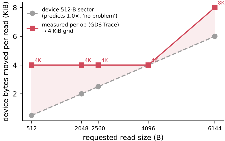
Per-op device bytes vs. the 512-B sector prediction
