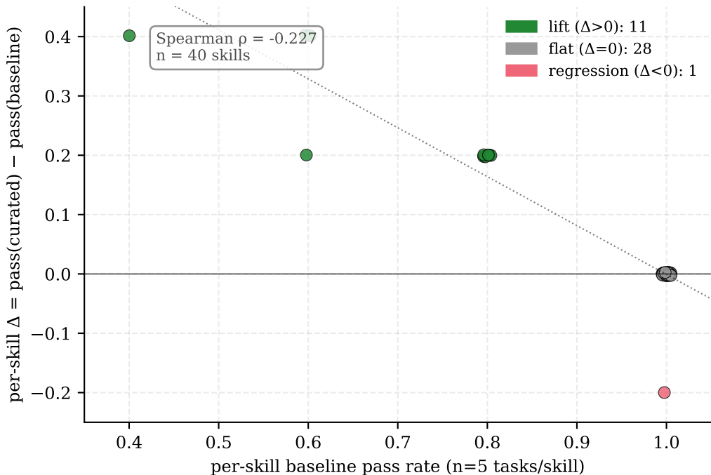
v2.0 per-skill: procedural- \Delta vs baseline pass rate (LLM-only judging)
