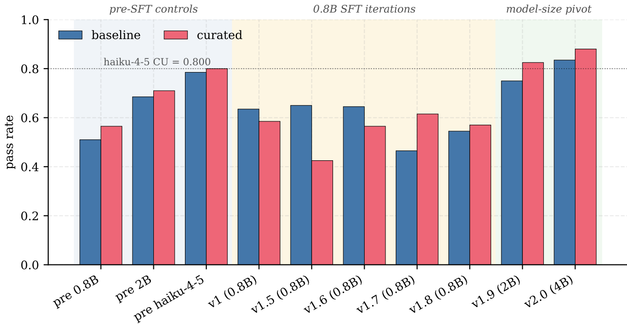
Baseline vs Curated pass rate across recipe variants and model scales
