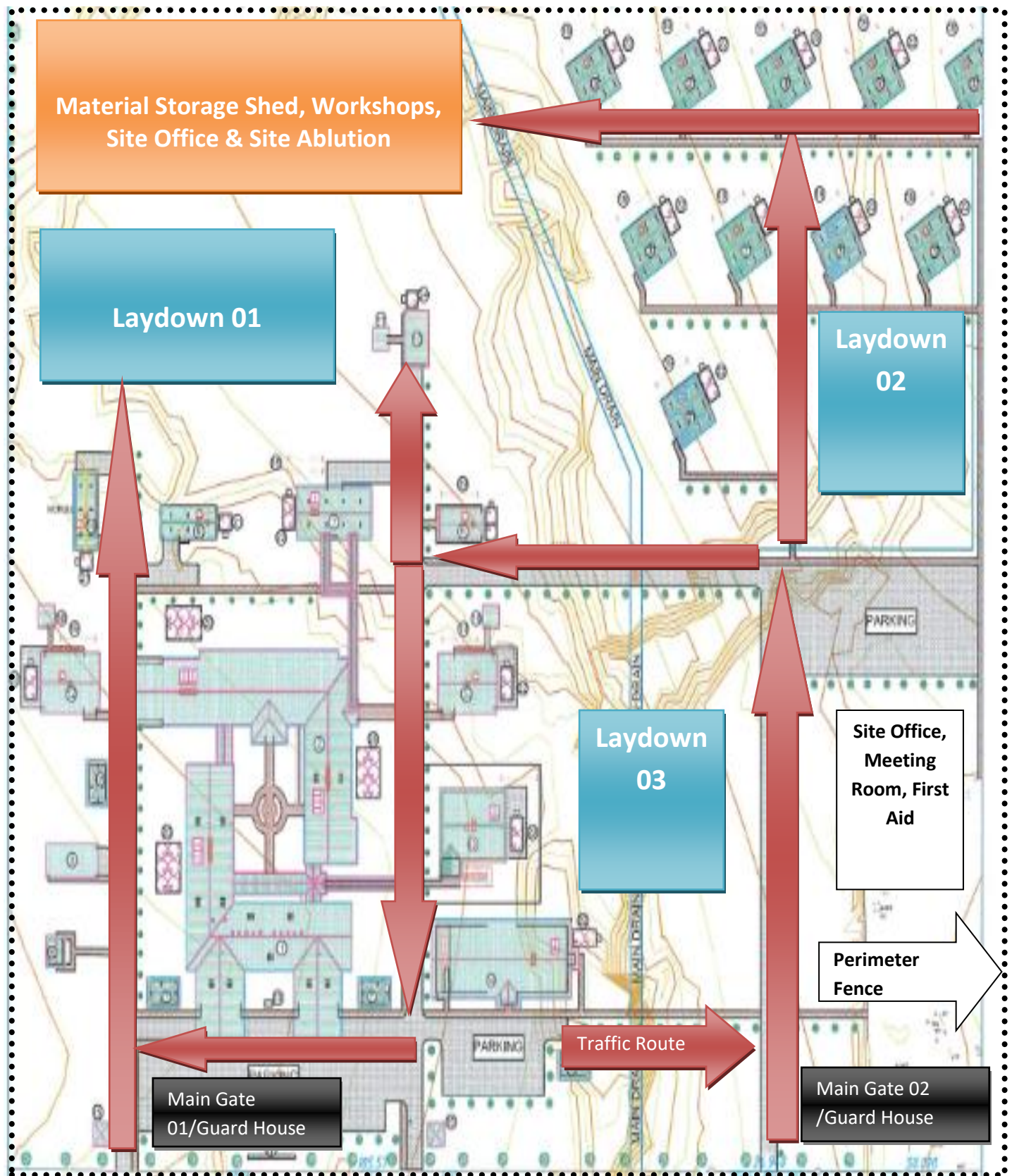
Figure 3. Proposed Site Layout
