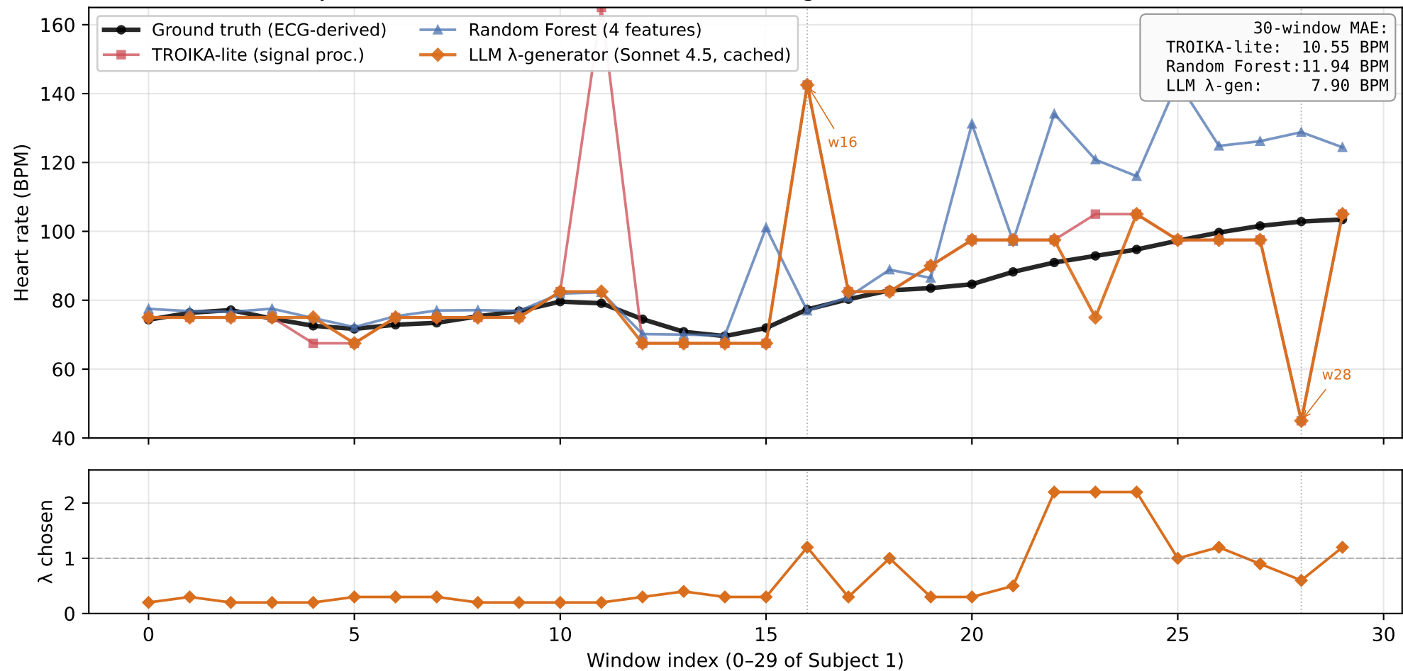
Subject 1 — first 30 windows: HR estimate vs ground truth (8 s windows, 2 s shift)
