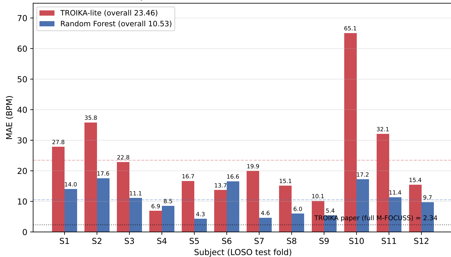
Per-subject HR estimation MAE — IEEE SPC 2015 (LOSO)
