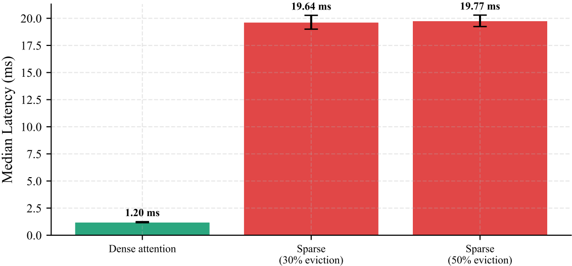
Kernel Timing — Kaggle TPU v5e-8
