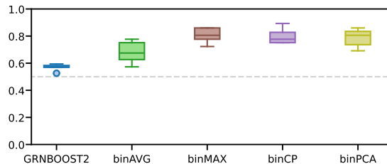
B undirected edges
