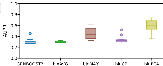
A directed edges
