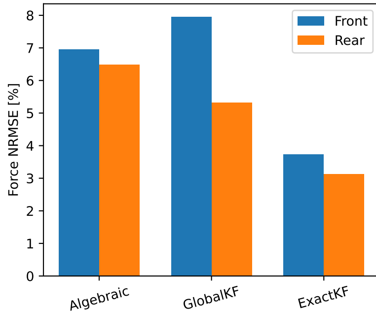
Tire-force estimation
