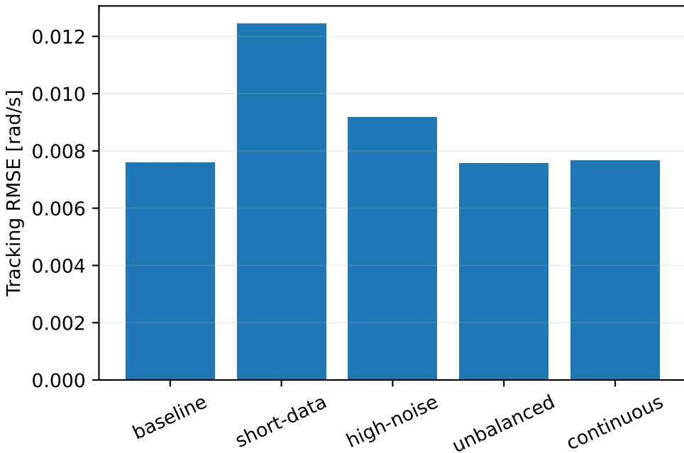
Learned-group control
