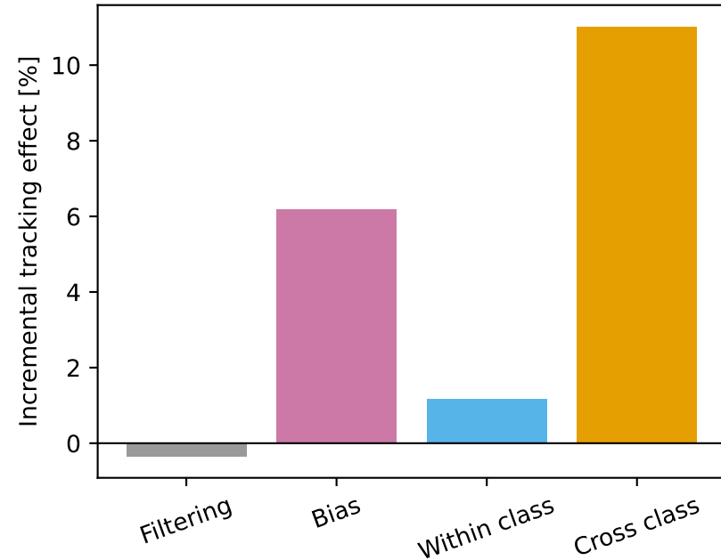
Transient mechanism attribution
