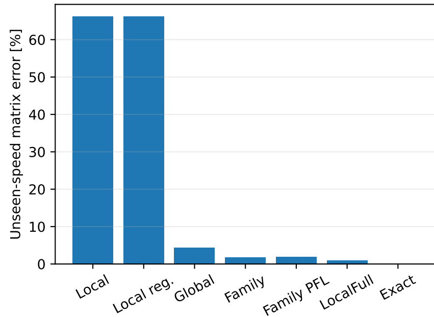
Finite-data prediction
