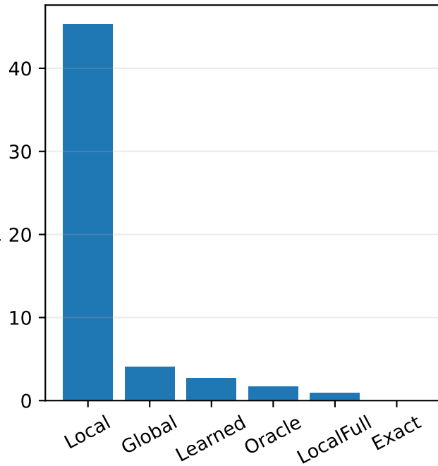
Full-envelope matrix error [%]
