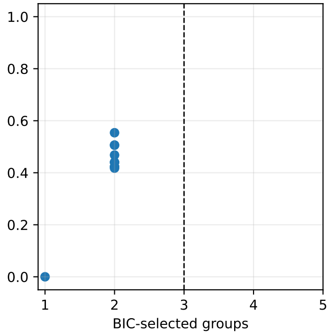
ARI
