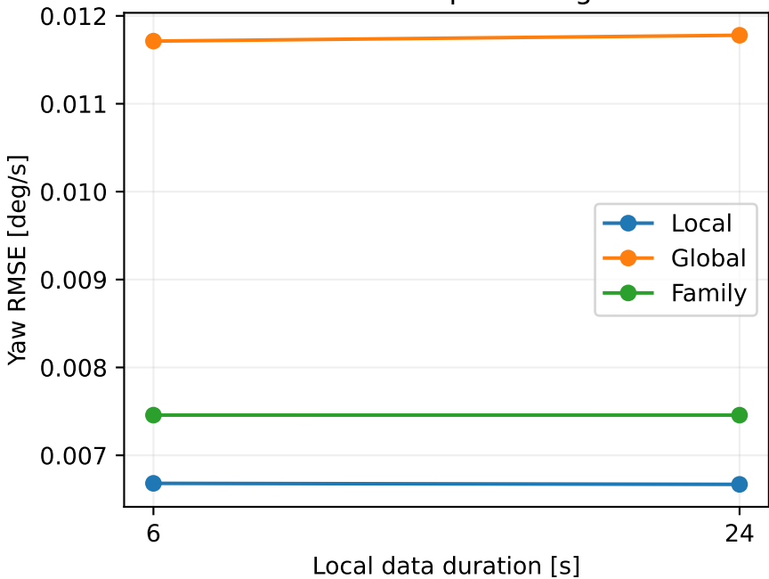
Closed-loop tracking
