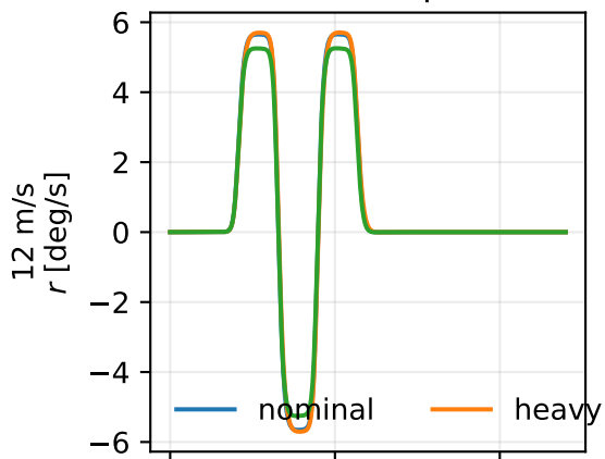
Yaw-rate response
