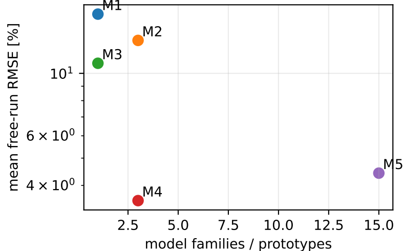
Accuracy--complexity view
