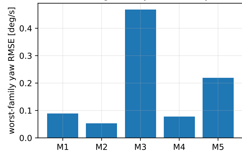
Redesign family consistency
