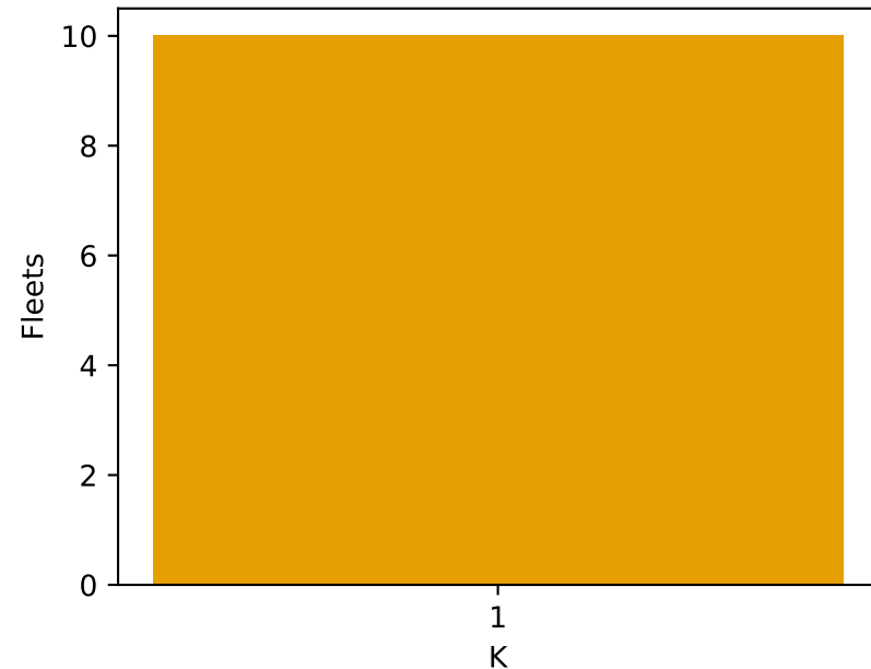
BIC-selected cardinality
