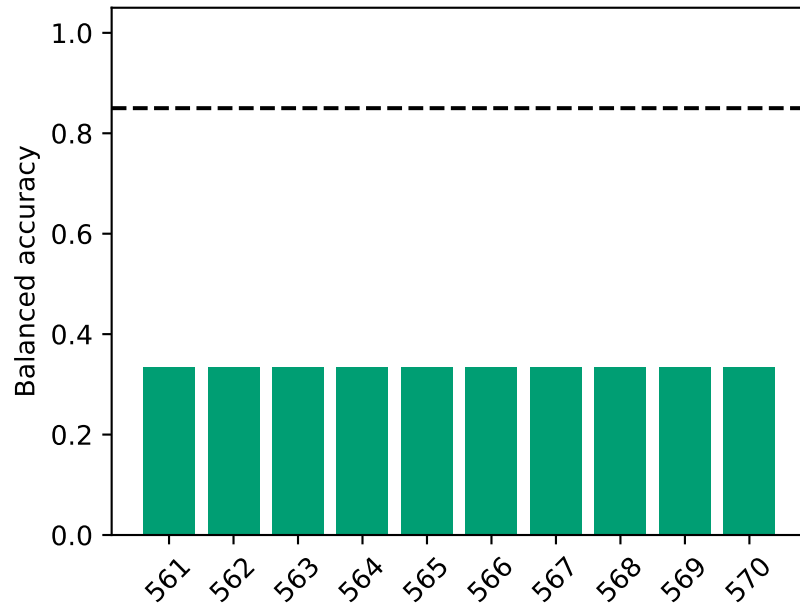
Permutation-matched assignment
