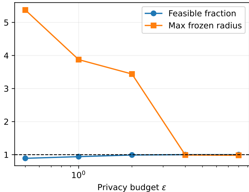
Safety diagnostics
