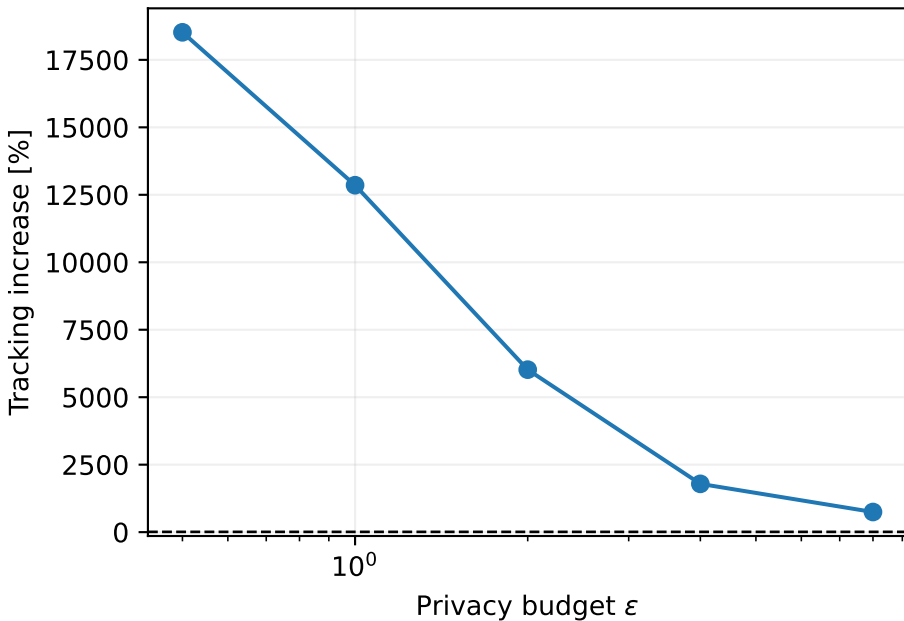
Privacy--control frontier
