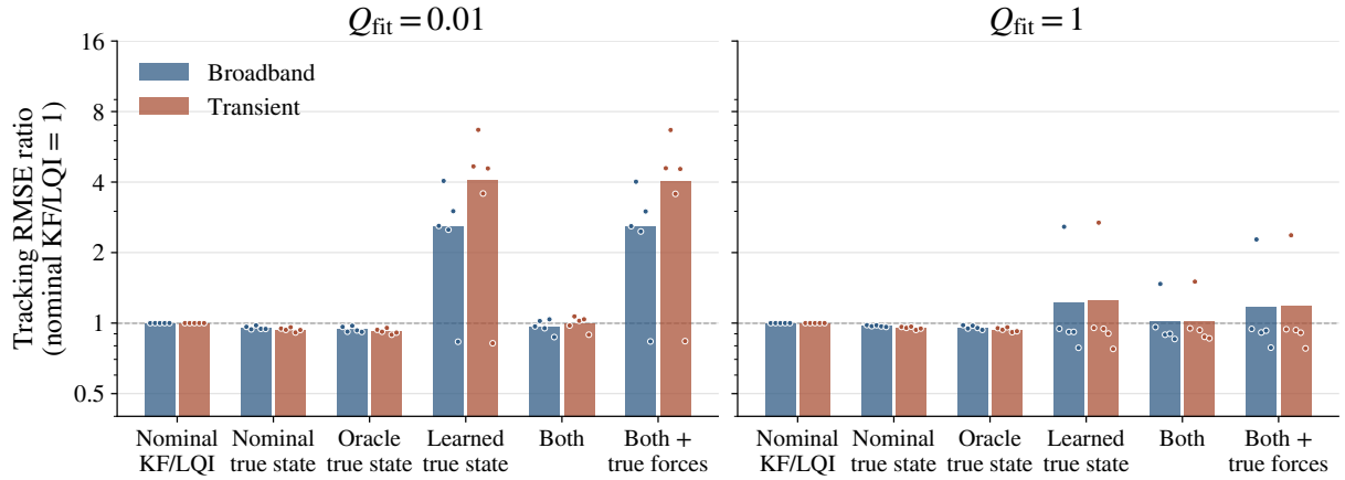
Figure 63: Frozen tracking diagnostic for both fitting panels. Bars are mean paired fleet RMSE ratios against nominal output feedback; dots retain all five fleets. The vertical axis is logarithmic. True states do not rescue the learned controller, and a harmful fleet tail remains visible in the comparison panel.
