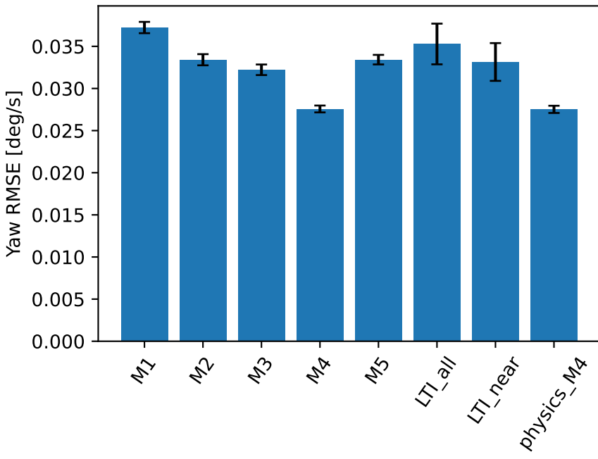
Independent fleets: mean and seed SD
